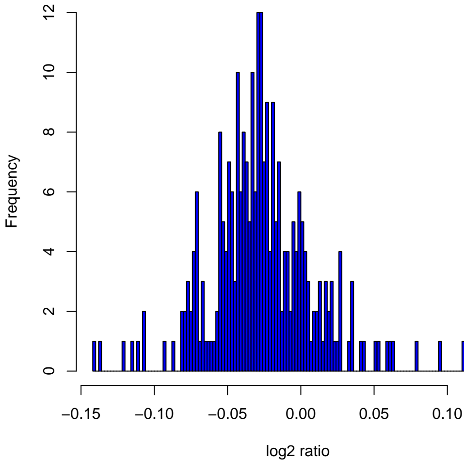
Histogram of log2ratios in 270 HapMap samples at clone Chr22tp-8B12
