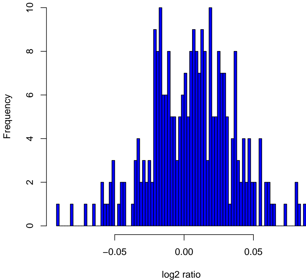
Histogram of log2ratios in 270 HapMap samples at clone Chr22tp-8C11
