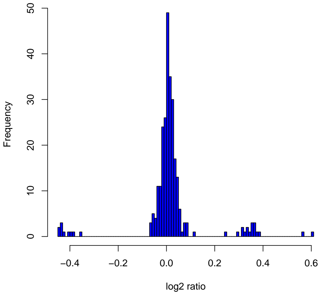
Histogram of log2ratios in 270 HapMap samples at clone Chr22tp-8G4
