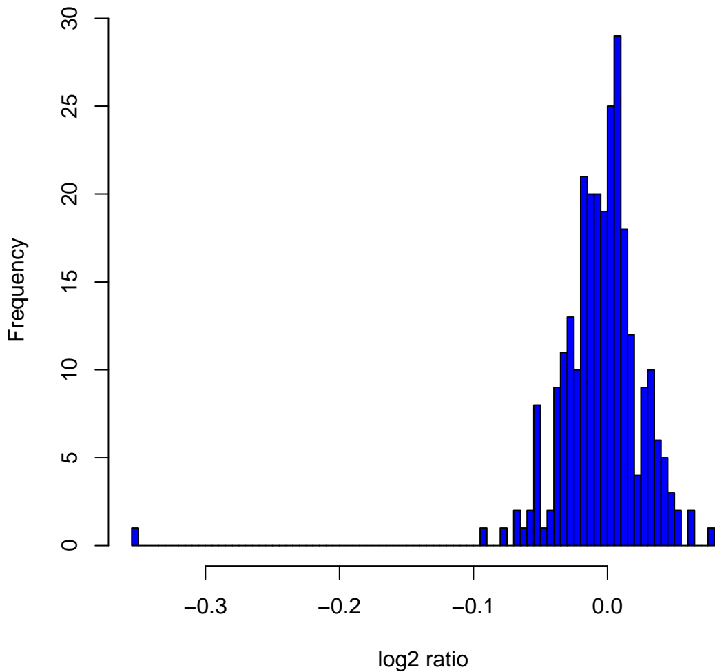
Histogram of log 2 ratios in 270 HapMap samples at clone Chr22tp-8H3
