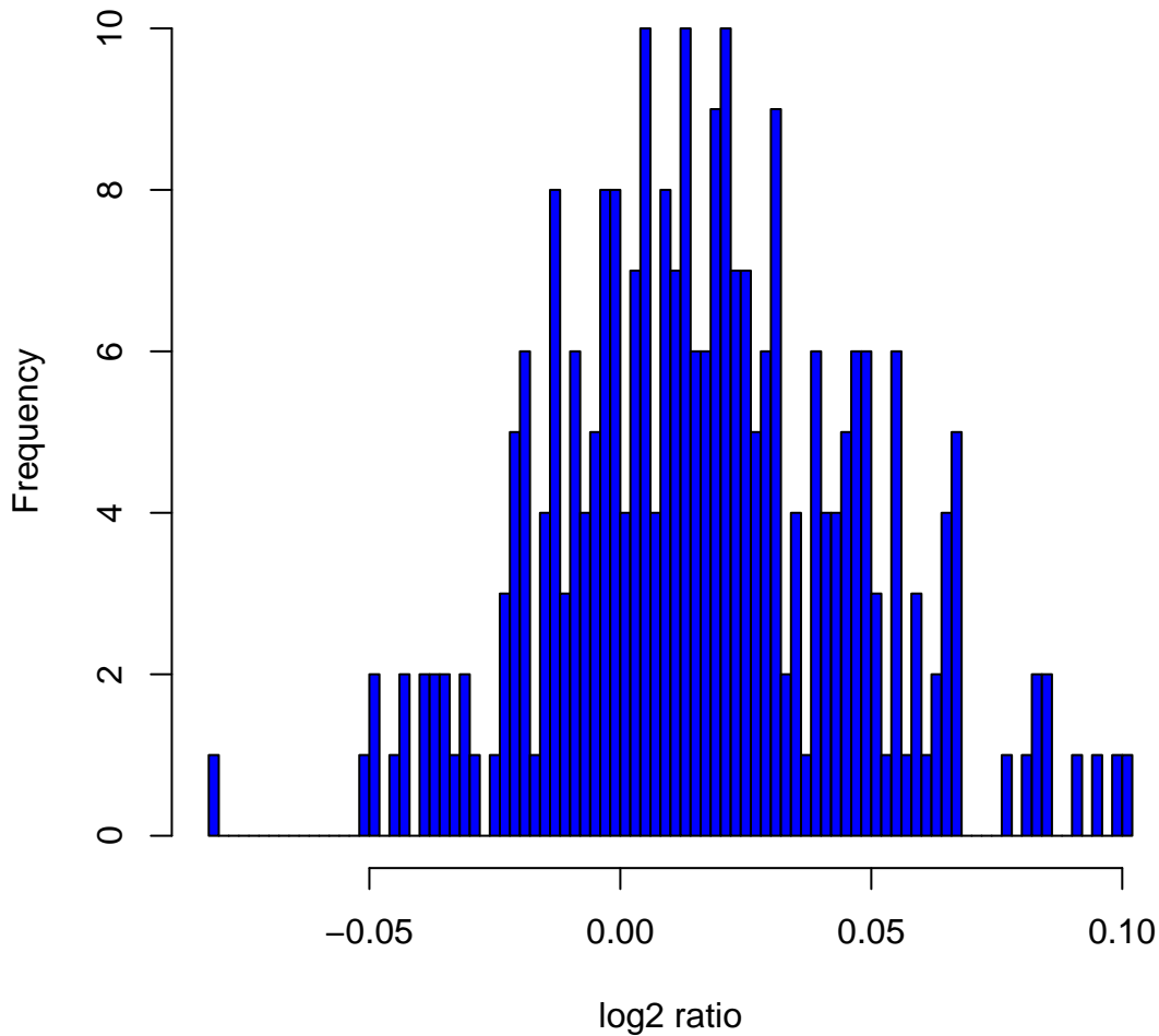
Histogram of log 2 ratios in 270 HapMap samples at clone Chr22tp-9C4
