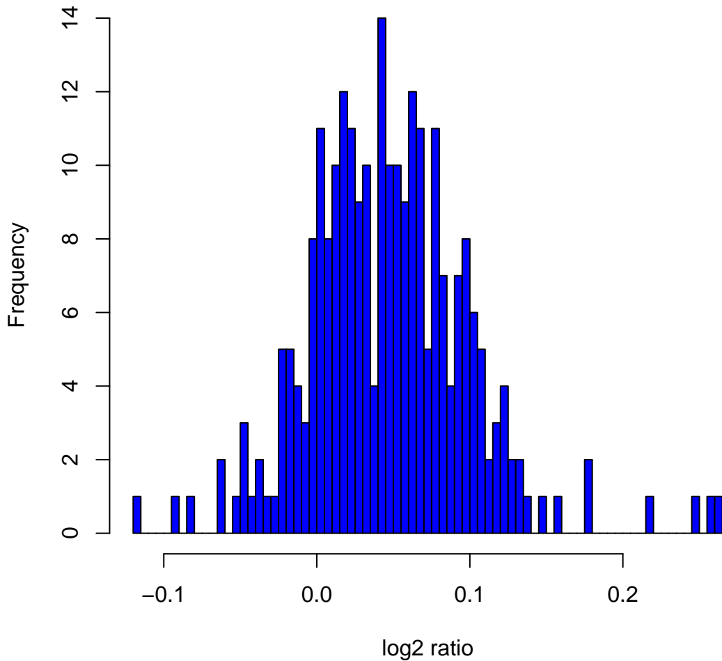
Histogram of log 2 ratios in 270 HapMap samples at clone Chr22tp-9F8
