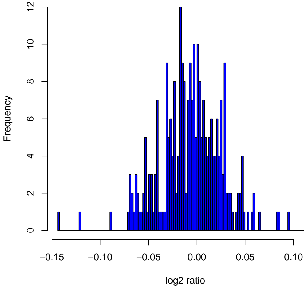
Histogram of log 2 ratios in 270 HapMap samples at clone Chr3tp-10D6
