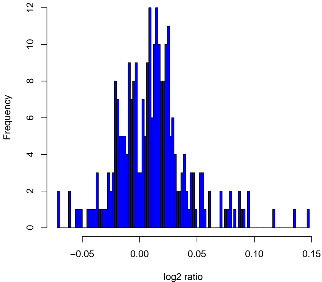
Histogram of log 2 ratios in 270 HapMap samples at clone Chr3tp-10G2
