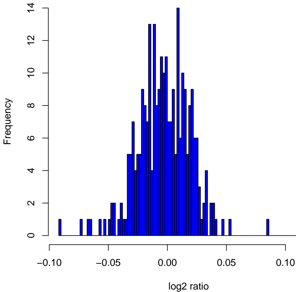
Histogram of \log_2 ratios in 270 HapMap samples at clone Chr3tp-10G4
