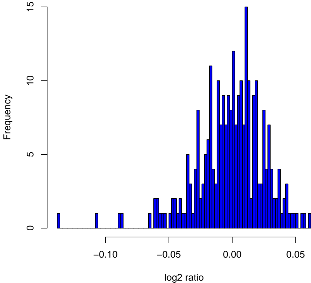
Histogram of log 2 ratios in 270 HapMap samples at clone Chr3tp-10G6
