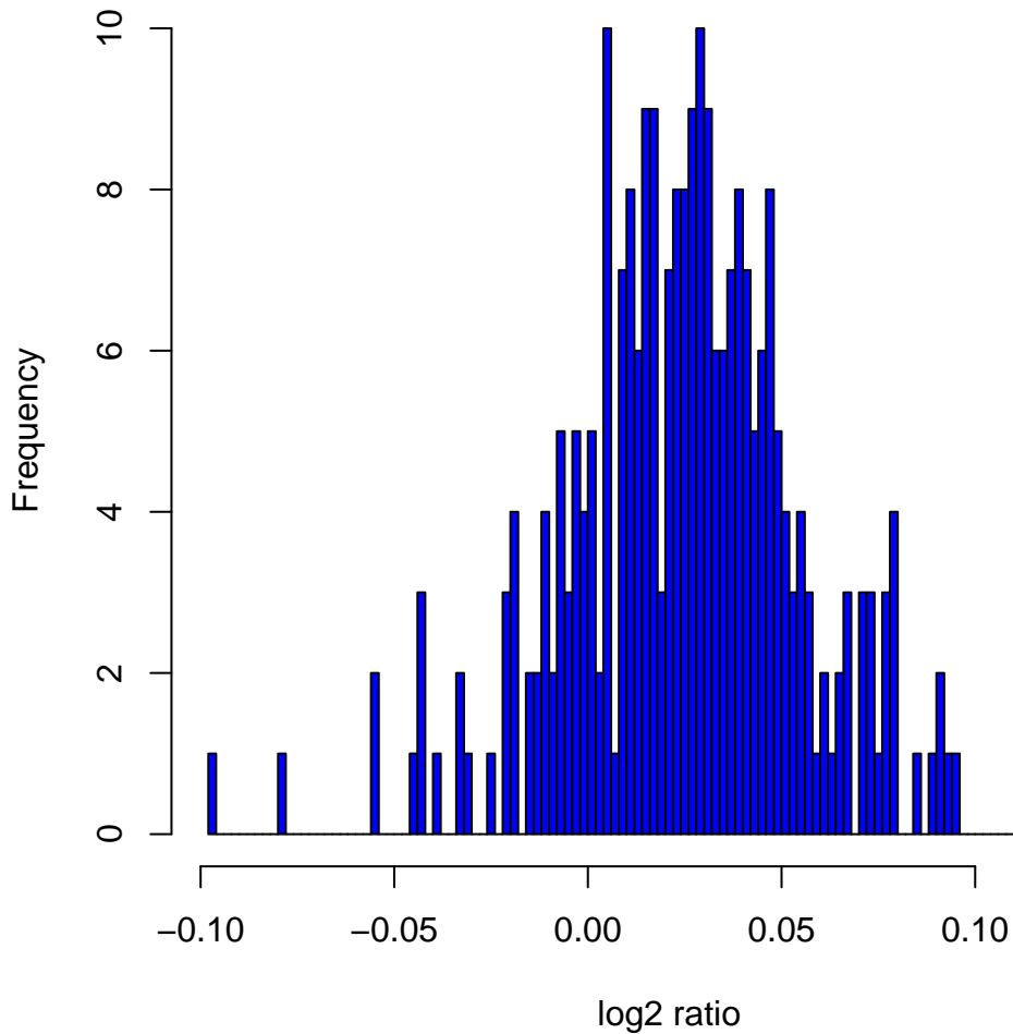
Histogram of log 2 ratios in 270 HapMap samples at clone Chr3tp-10H3
