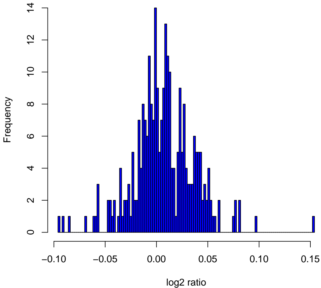
Histogram of \log_2 ratios in 270 HapMap samples at clone Chr3tp-11C1
