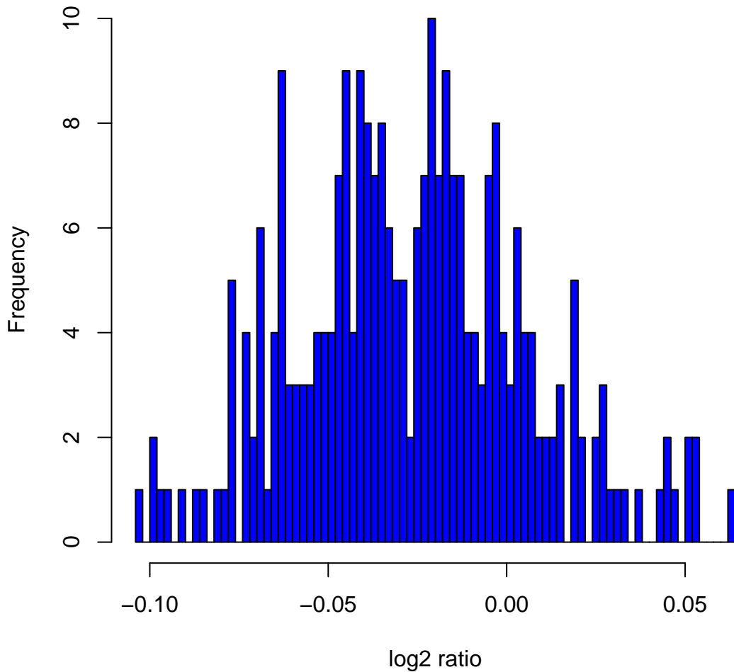
Histogram of log2ratios in 270 HapMap samples at clone Chr3tp-11C10
