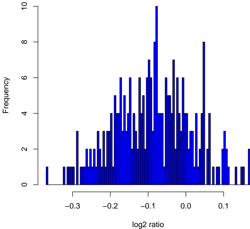
Histogram of log2ratios in 270 HapMap samples at clone Chr3tp-11C6
