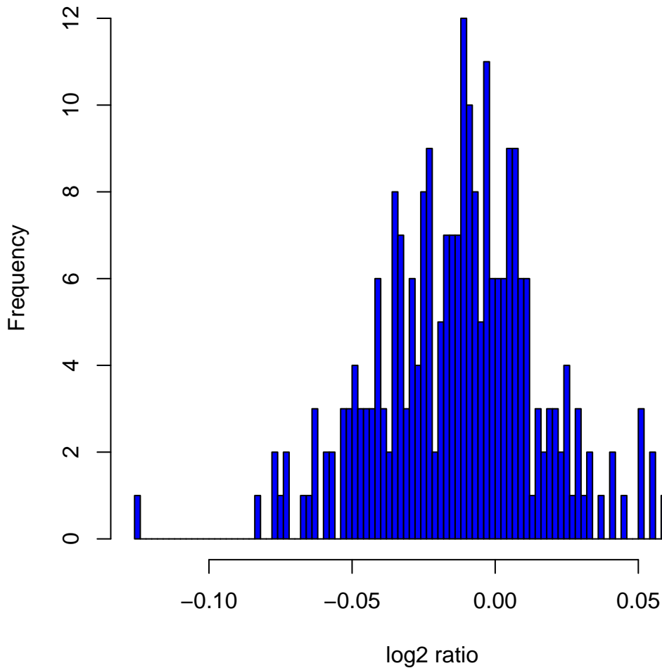
Histogram of log 2 ratios in 270 HapMap samples at clone Chr3tp-11F6
