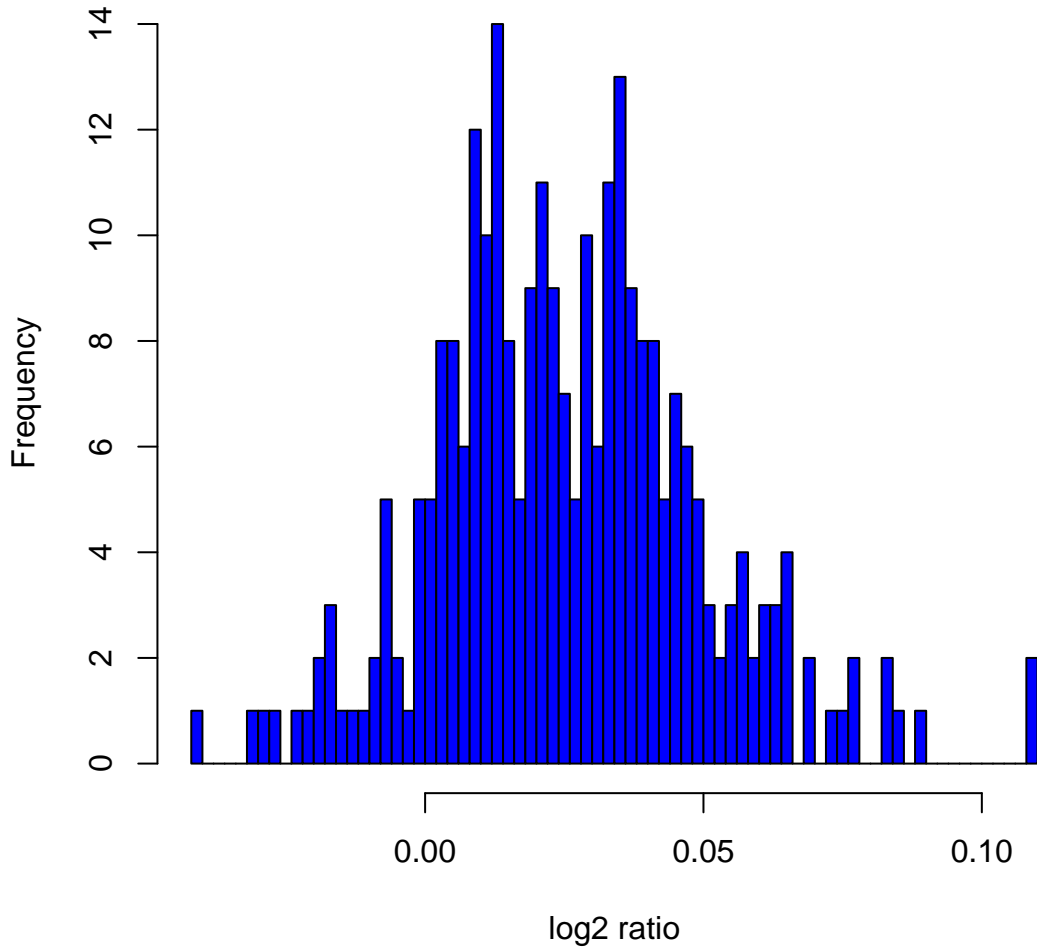
Histogram of log2ratios in 270 HapMap samples at clone Chr3tp-12B11
