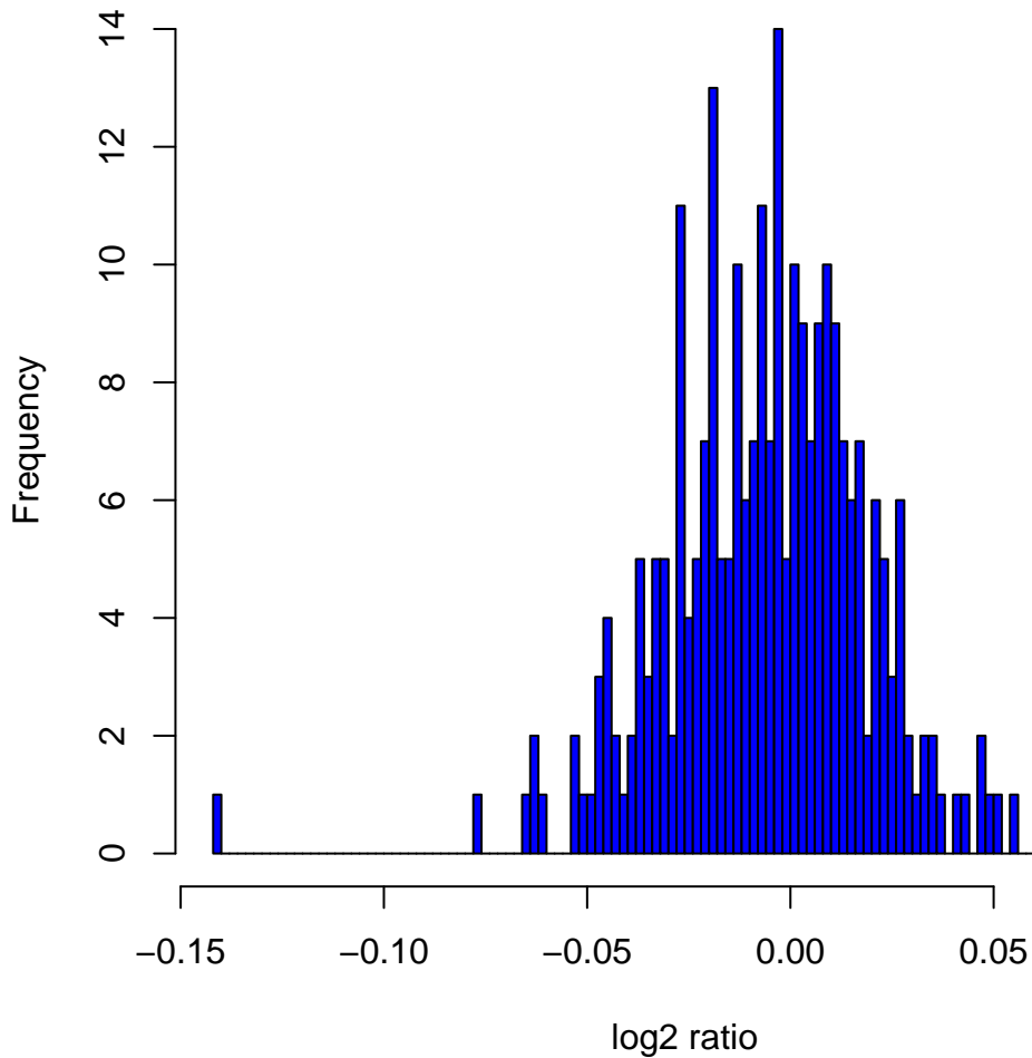
Histogram of log 2 ratios in 270 HapMap samples at clone Chr3tp-13B1
