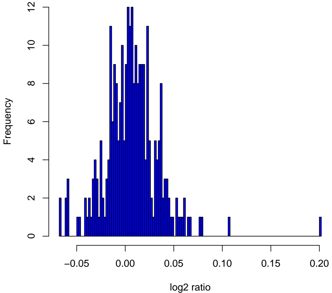
Histogram of \log_2 ratios in 270 HapMap samples at clone Chr3tp-14C4
