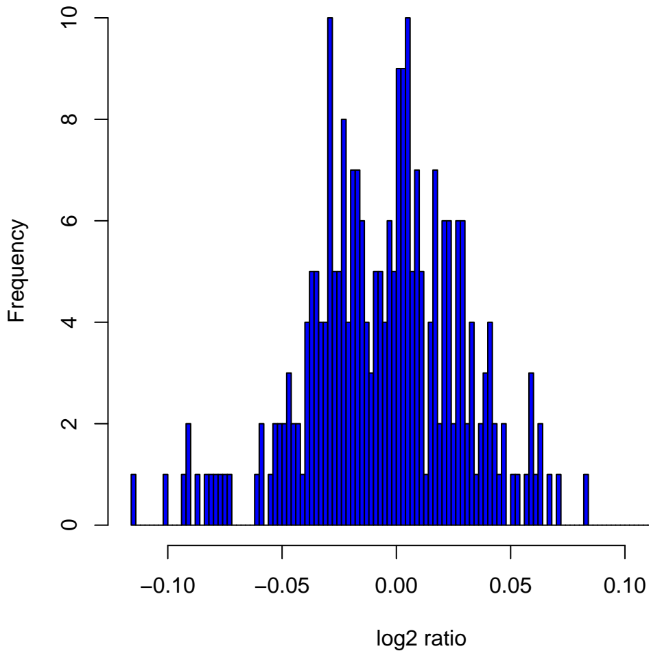
Histogram of \log_2 ratios in 270 HapMap samples at clone Chr3tp-14D1
