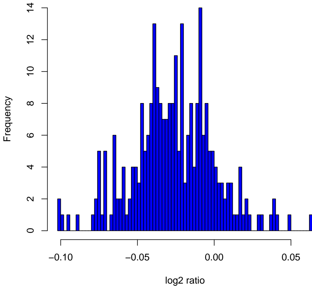
Histogram of log 2 ratios in 270 HapMap samples at clone Chr3tp-14E3
