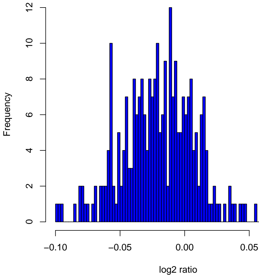
Histogram of \log_2 ratios in 270 HapMap samples at clone Chr3tp-14G3
