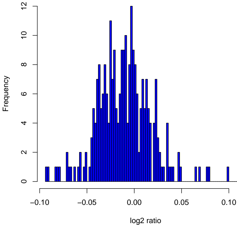
Histogram of log 2 ratios in 270 HapMap samples at clone Chr3tp-15F1
