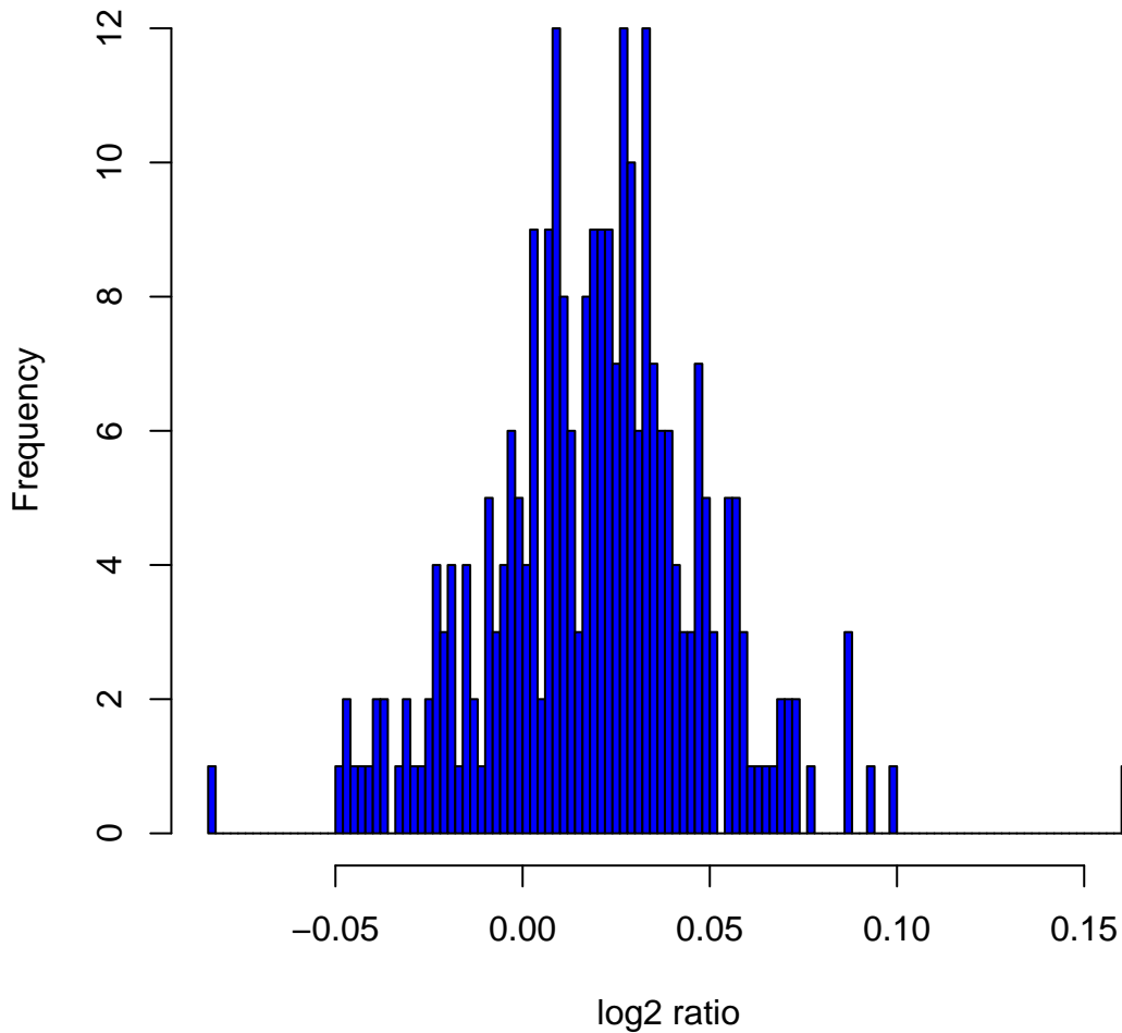
Histogram of log 2 ratios in 270 HapMap samples at clone Chr3tp-15F9
