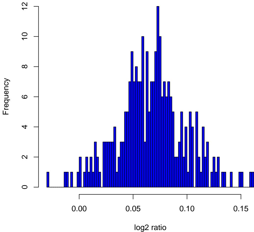
Histogram of log2ratios in 270 HapMap samples at clone Chr3tp-15G10
