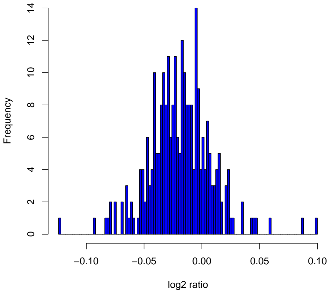
Histogram of log 2 ratios in 270 HapMap samples at clone Chr3tp-15G6
