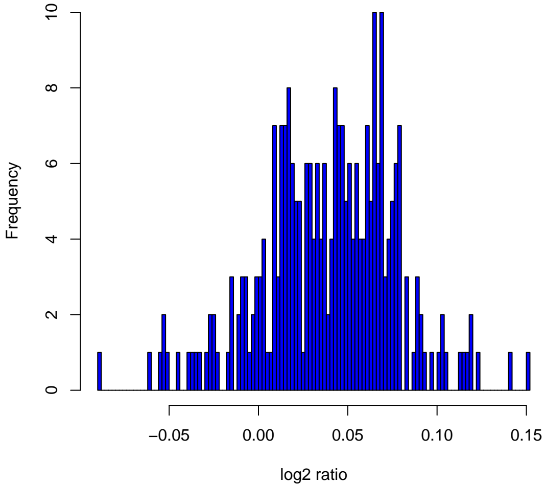
Histogram of log 2 ratios in 270 HapMap samples at clone Chr3tp-15G7
