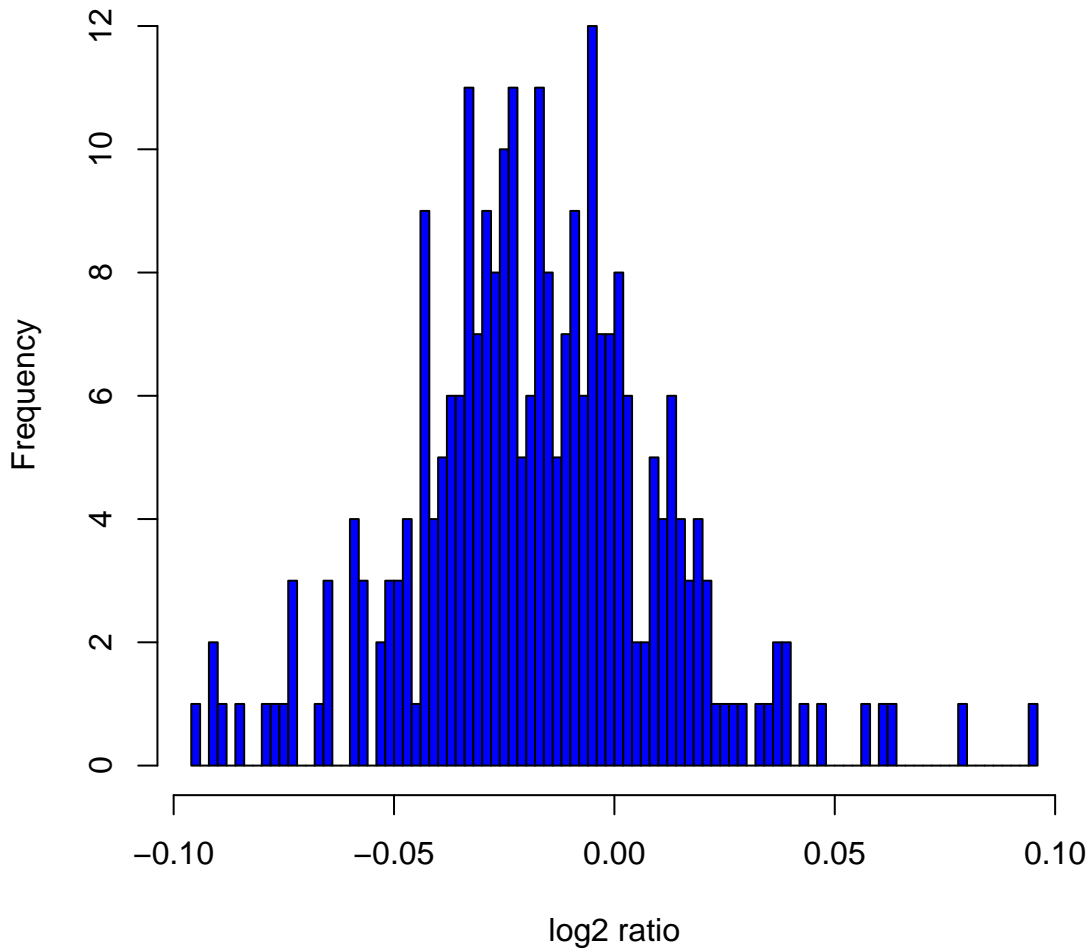
Histogram of log2ratios in 270 HapMap samples at clone Chr3tp-16A12
