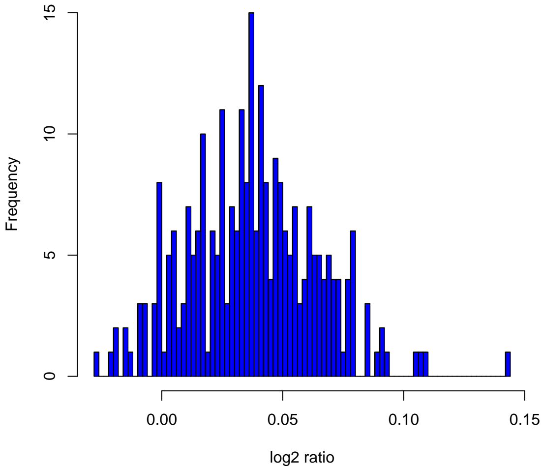
Histogram of log2ratios in 270 HapMap samples at clone Chr3tp-16E11
