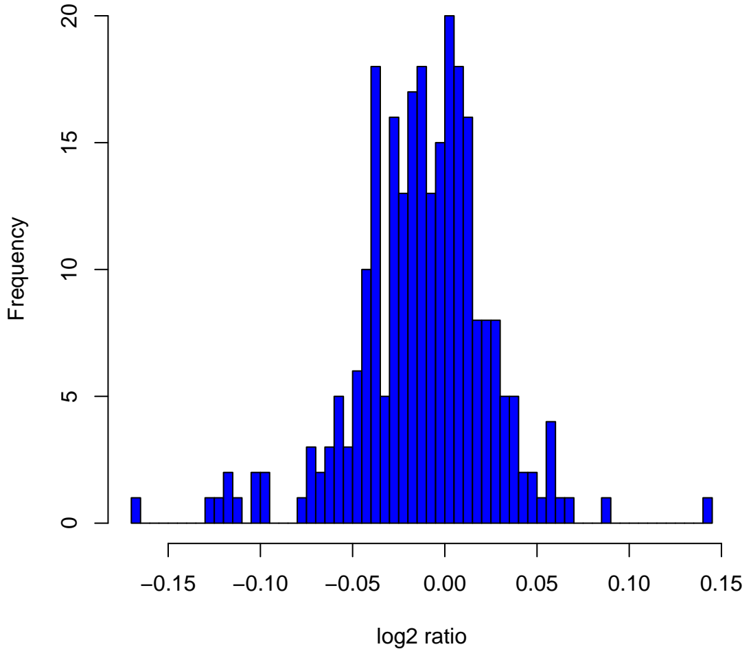
Histogram of log 2 ratios in 270 HapMap samples at clone Chr3tp-16H2
