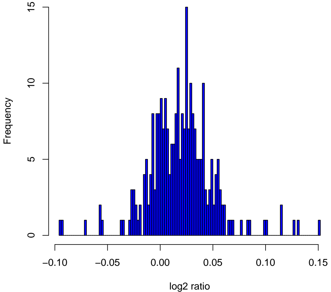
Histogram of log 2 ratios in 270 HapMap samples at clone Chr3tp-17C7
