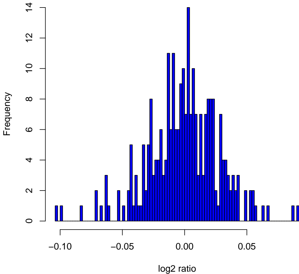
Histogram of \log_2 ratios in 270 HapMap samples at clone Chr3tp-17D12
