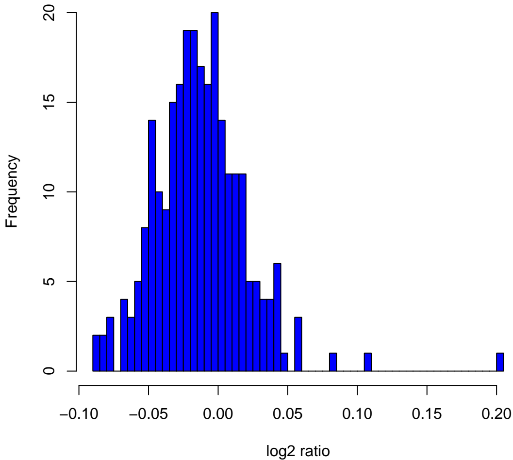
Histogram of log2ratios in 270 HapMap samples at clone Chr3tp-17F11
