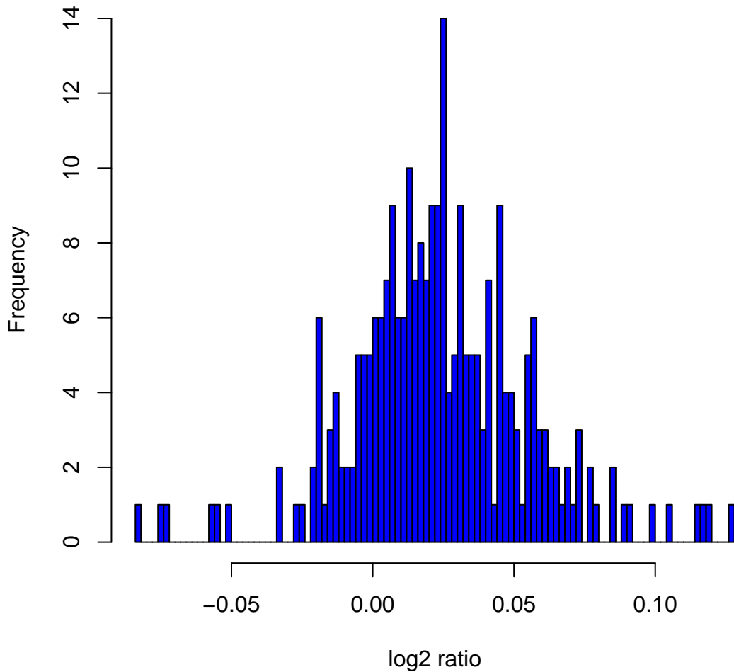
Histogram of log2ratios in 270 HapMap samples at clone Chr3tp-17F12
