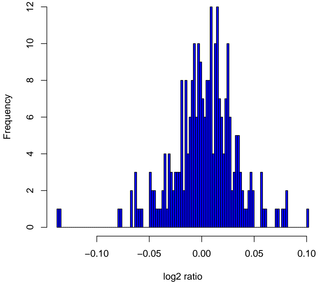
Histogram of log2ratios in 270 HapMap samples at clone Chr3tp-18C11
