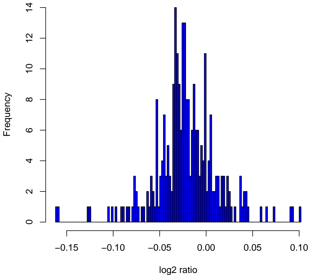
Histogram of log2ratios in 270 HapMap samples at clone Chr3tp-18C12
