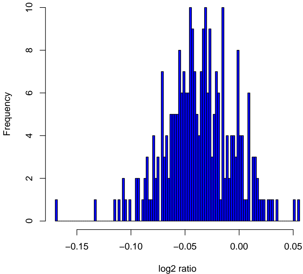
Histogram of log 2 ratios in 270 HapMap samples at clone Chr3tp-18C6
