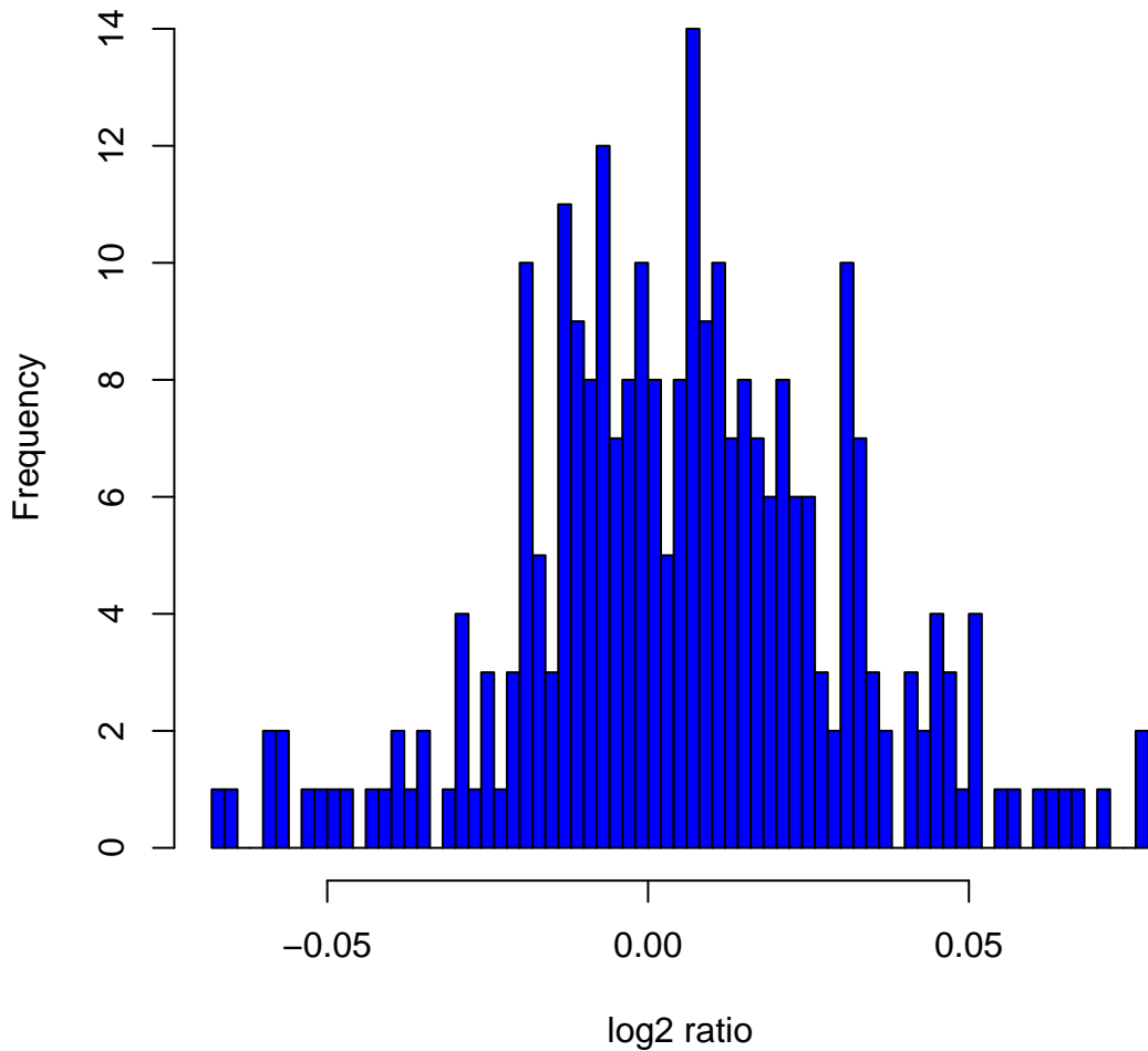
Histogram of log 2 ratios in 270 HapMap samples at clone Chr3tp-18D2
