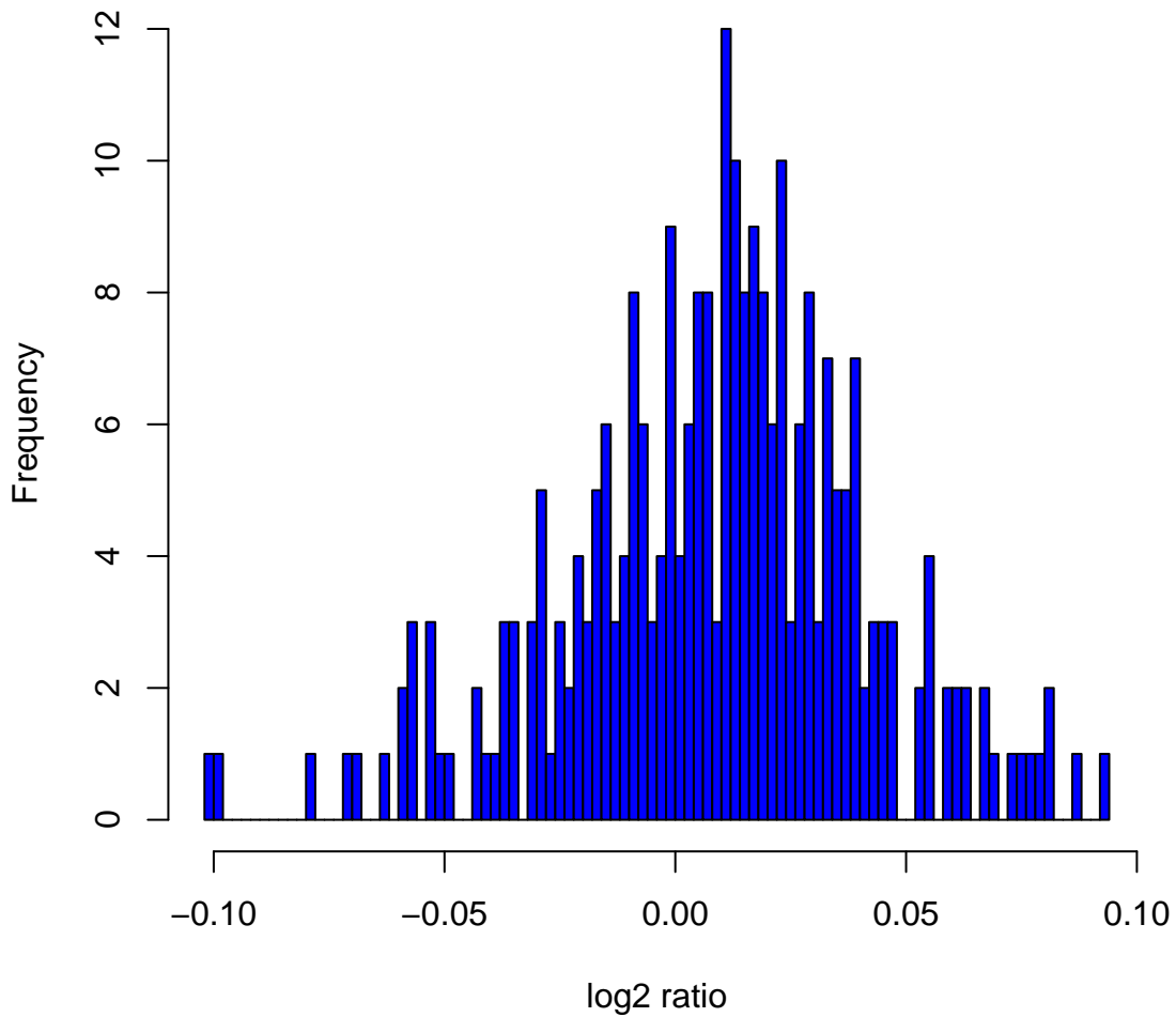
Histogram of log 2 ratios in 270 HapMap samples at clone Chr3tp-18D7
