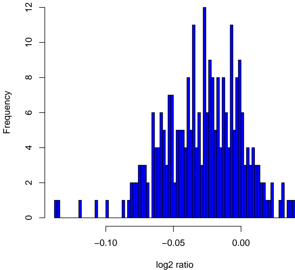
Histogram of log2ratios in 270 HapMap samples at clone Chr3tp-19H12
