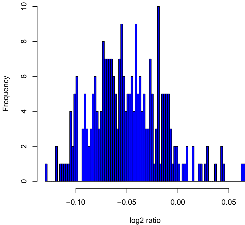
Histogram of log 2 ratios in 270 HapMap samples at clone Chr3tp-19H6
