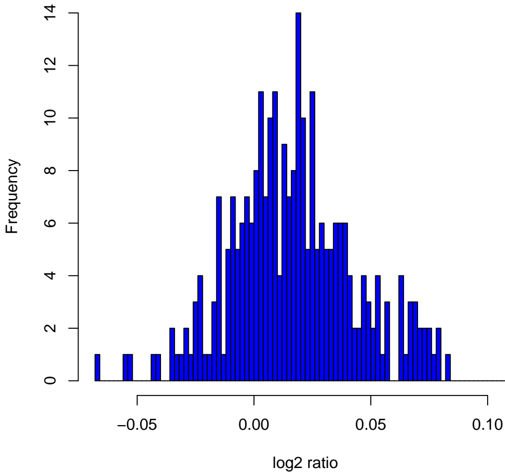
Histogram of \log_2 ratios in 270 HapMap samples at clone Chr3tp-1B6
