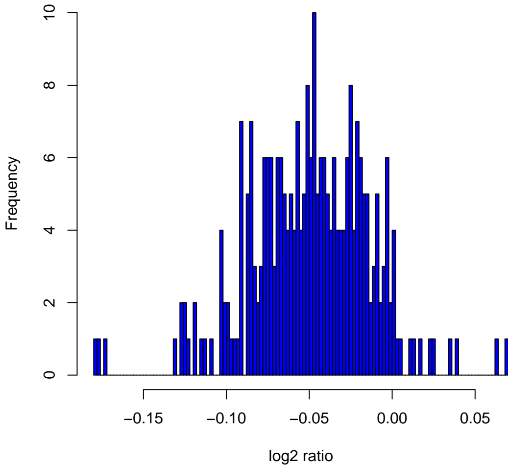
Histogram of \log_2 ratios in 270 HapMap samples at clone Chr3tp-1D5
