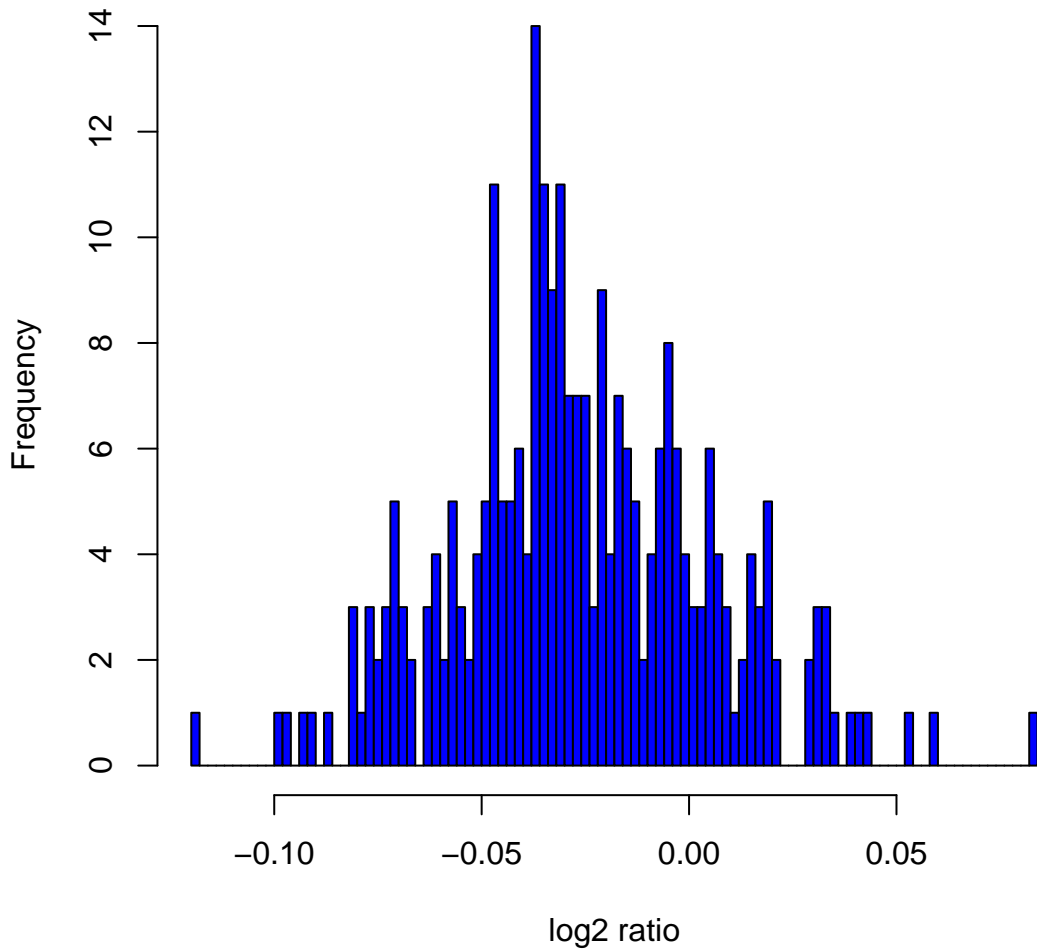
Histogram of log 2 ratios in 270 HapMap samples at clone Chr3tp-1E7
