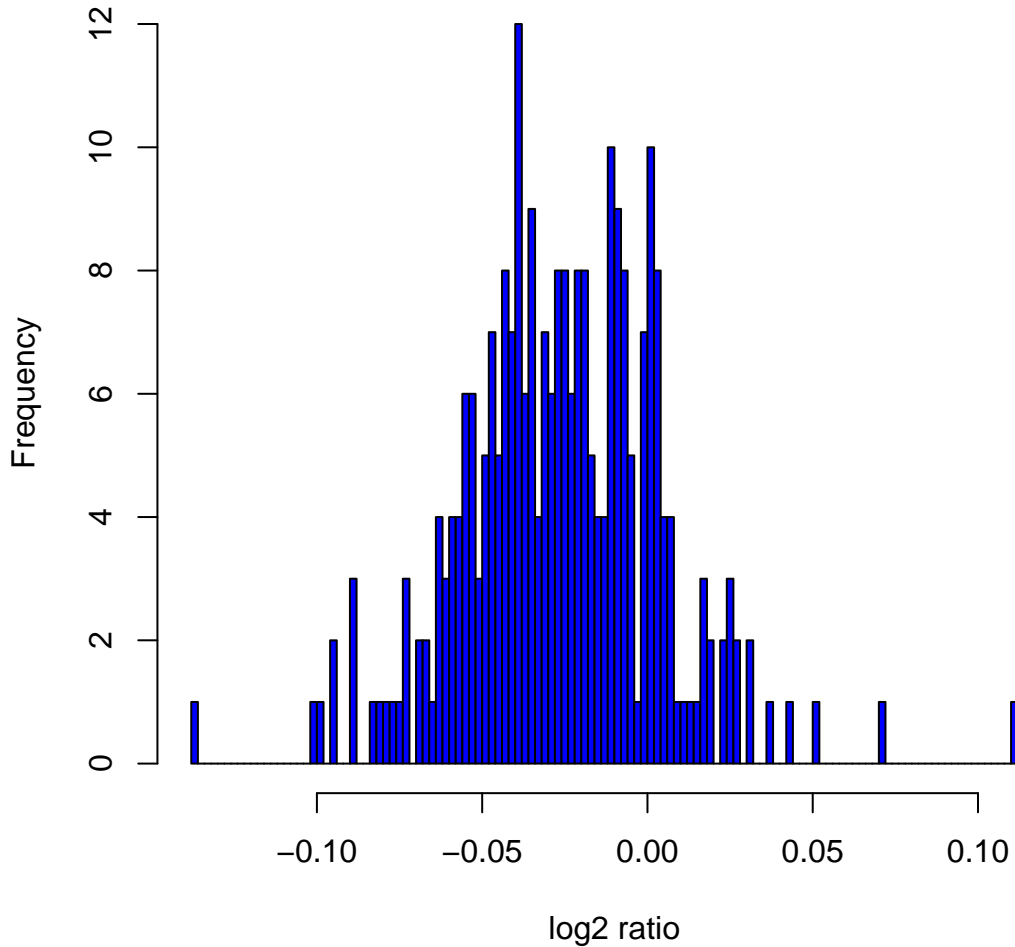
Histogram of log2ratios in 270 HapMap samples at clone Chr3tp-1F4
