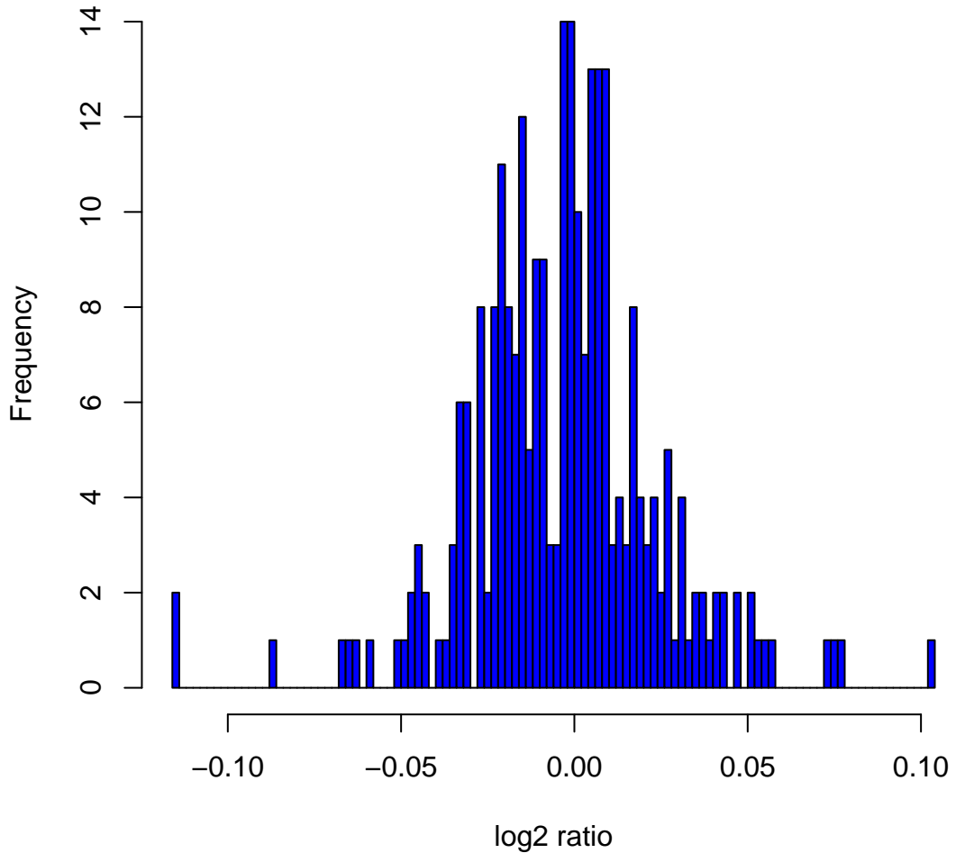
Histogram of log 2 ratios in 270 HapMap samples at clone Chr3tp-20A3
