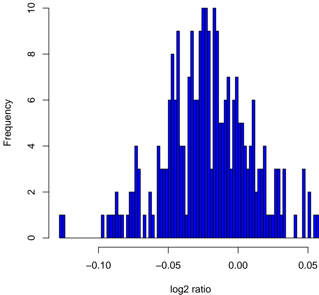
Histogram of log2ratios in 270 HapMap samples at clone Chr3tp-20C12
