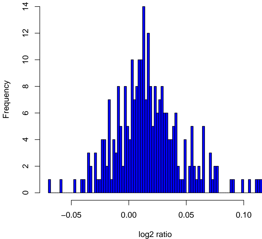
Histogram of \log_2 ratios in 270 HapMap samples at clone Chr3tp-20H2
