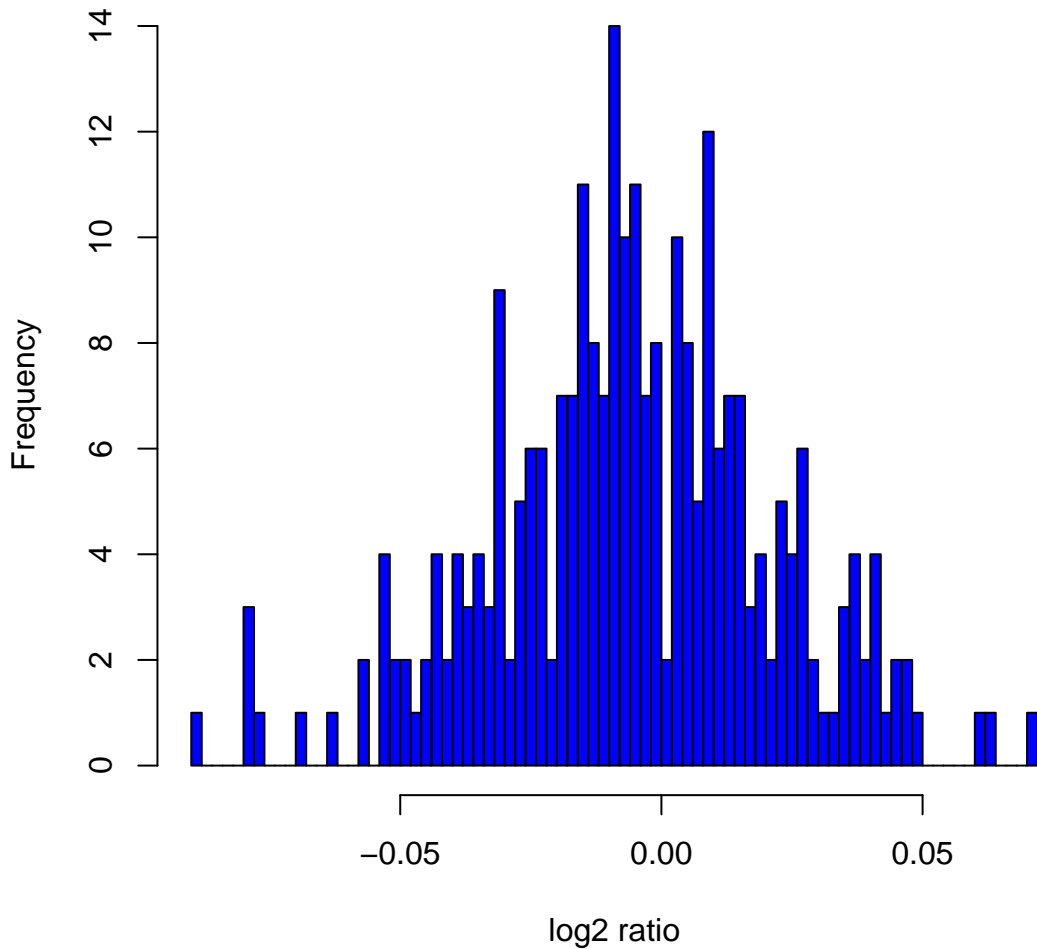
Histogram of log 2 ratios in 270 HapMap samples at clone Chr3tp-21B5
