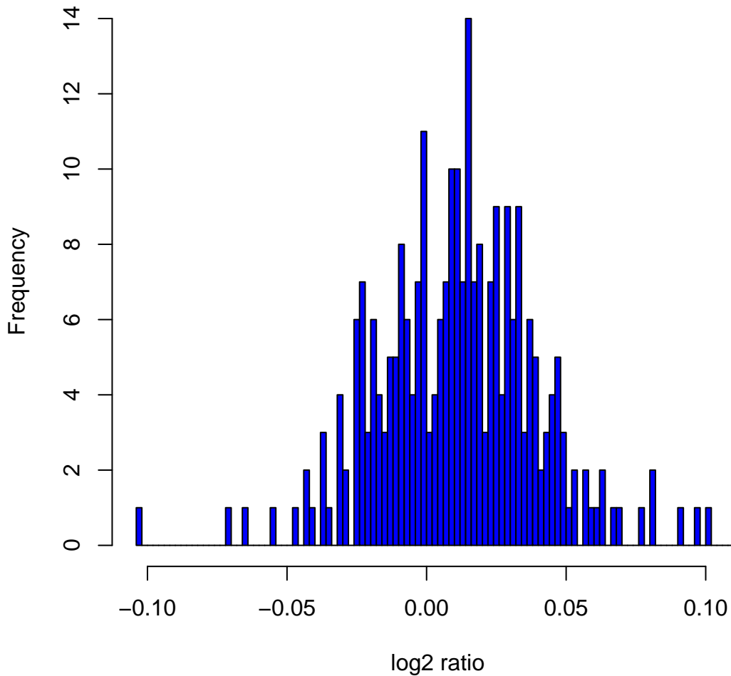
Histogram of log2ratios in 270 HapMap samples at clone Chr3tp-21C10
