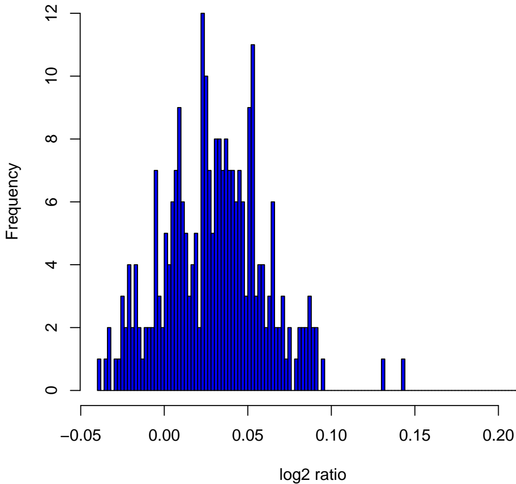
Histogram of log 2 ratios in 270 HapMap samples at clone Chr3tp-22A2
